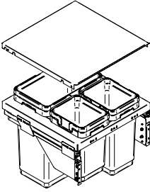
M 50 PGTM503RF (30+10+9) Lt
