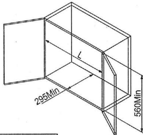
B. Double-door structure
